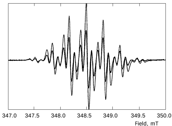
FIG. 5 SEESR; first-derivative ESR spectrum of the radical cation of 5 \cdot 10^{-3} M 1,4-di- tert -butyl-2,5-dimethoxybenzene in \text{CH}_3\text{CN} with 0.1 M TBAP, [\mathbf{1}]^{+\bullet} generated by electrolysis in situ at a Pt electrode; g = 2.0031 , a(^1\text{H}) = 0.322 mT (6 H), a(^1\text{H}) = 0.100 mT (2 H), solid line experimental, dotted line simulated
