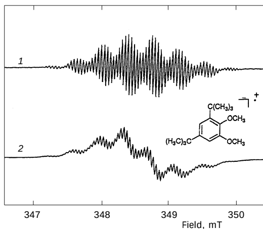
FIG. 6 SEESR; first-derivative of in situ ESR spectrum obtained during electrolysis at 20(\pm 1)^\circ\text{C} (Pt electrode) in \text{CH}_3\text{CN} containing 0.1 M TBAP and 3,5-di- tert -butyl-1,2-dimethoxybenzene ( 2 ) of concentrations: (1) 5, (2) 30 mmol \text{l}^{-1} . The modulation amplitude is 0.02 mT and modulation frequency 50 kHz; g = 2.0032(\pm 0.0001)
